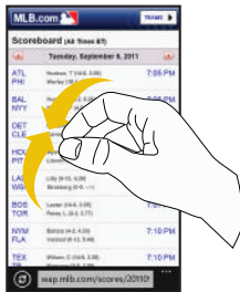
Zoom Out
