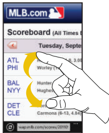
Zoom In
